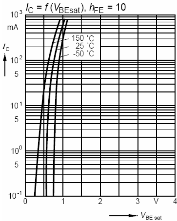
Base-emitter saturation voltage
