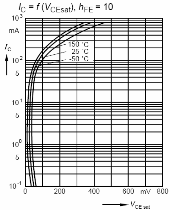
Collector-emitter saturation voltage
